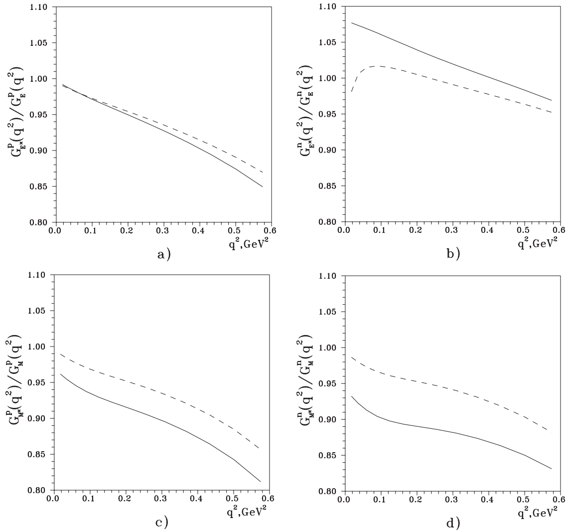
Fig. 2. Form factors normalized to their free-space values for two densities within the {}^4\text{He} nucleus. The distance of the center of the nucleon from the center of the nucleus is 0 fm (solid lines) and 1 fm (dashed lines). Panels a), b) c) and d) give the proton electric, neutron electric, proton magnetic and neutron magnetic form factors, in order.
