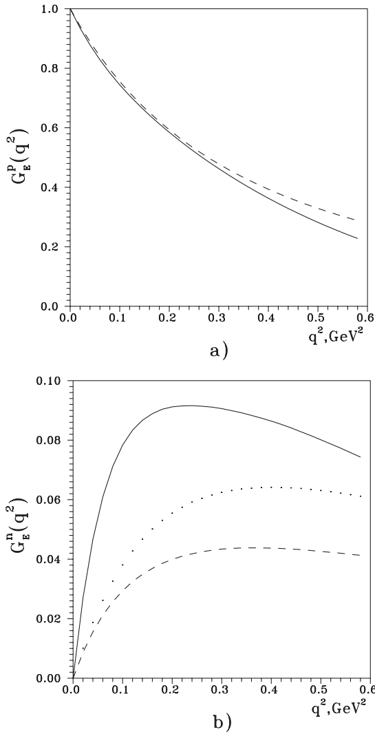
Fig. 1. Electric proton (a) and electric neutron (b) form factor. Solid (dashed) lines: our model (dispersion-theoretical analysis of [12]). The dotted line in G_E^n(q^2) represents the parametrization equation (19).
